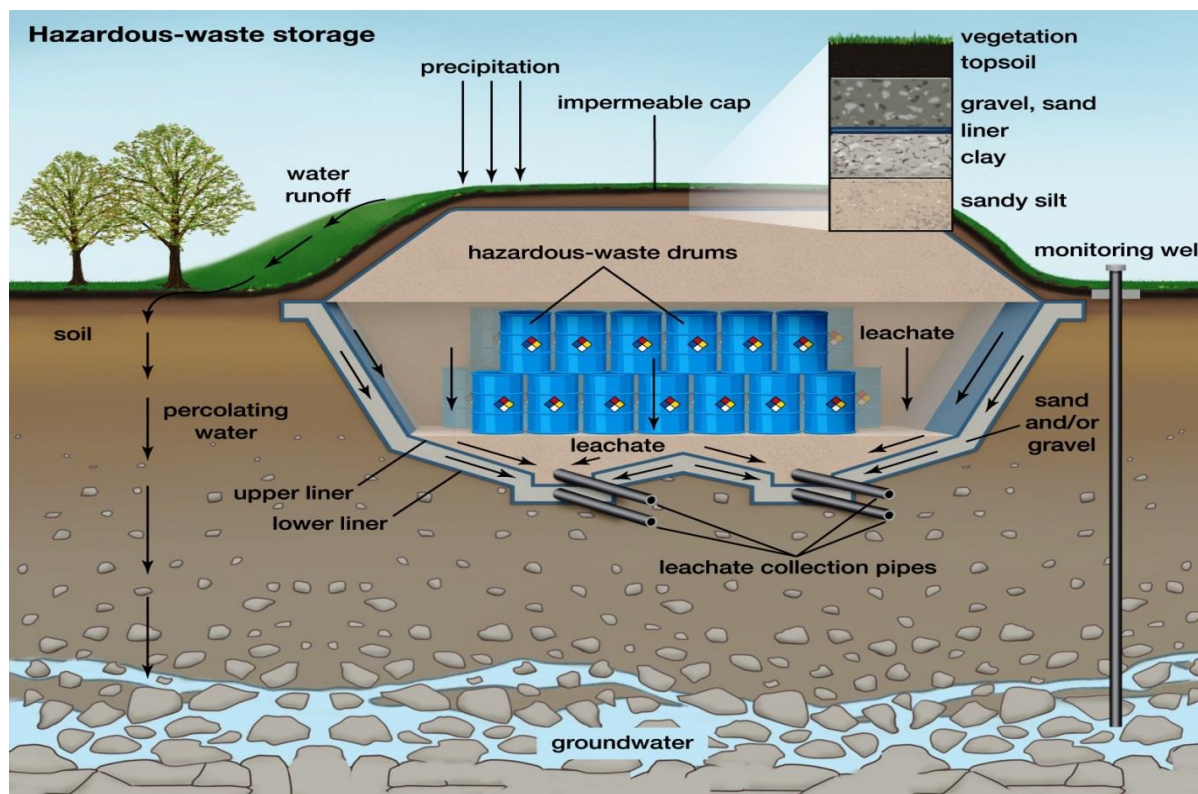
Fig.1 - Hazardous-waste management - Treatment, storage, and disposal
